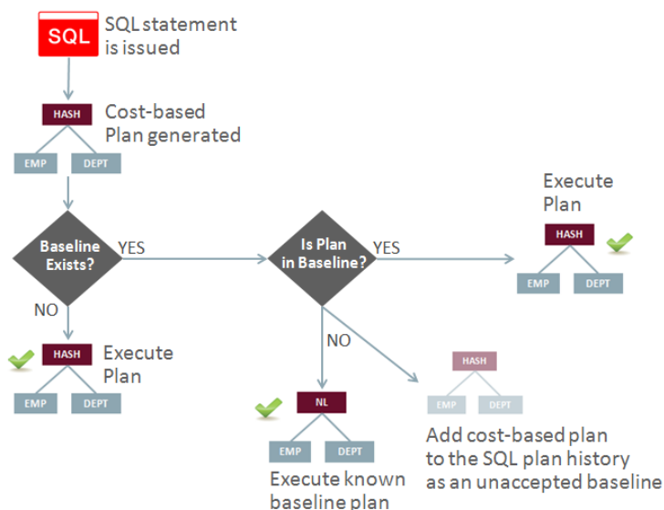
Figure 3: Flowchart of how plan selection works.
